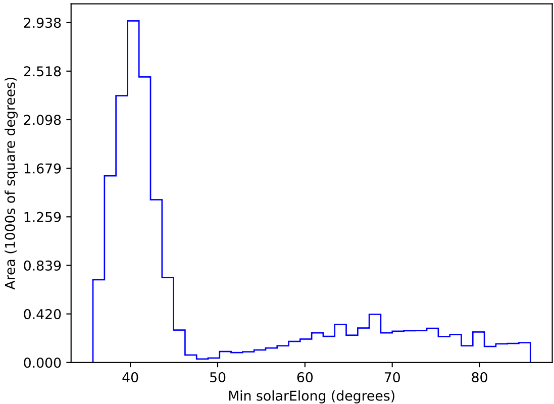
too_elab_heavy_r32_d3_gz_v3.4_10yrs WFD i band: Min solarElong
