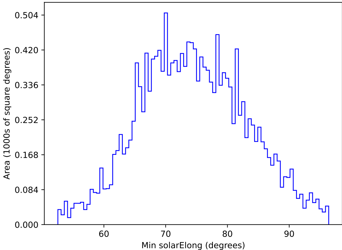
too_elab_heavy_r32_d3_gz_v3.4_10yrs WFD g band: Min solarElong
