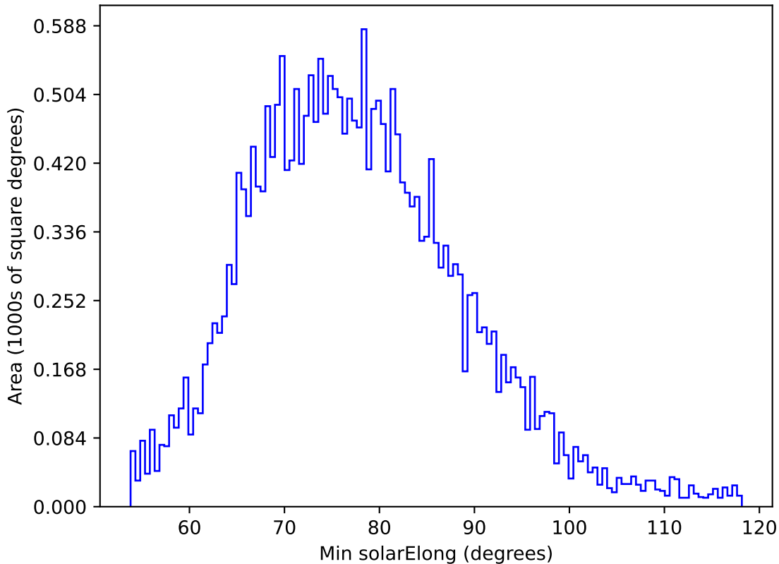
too_elab_heavy_r32_d3_gz_v3.4_10yrs All sky g band: Min solarElong
