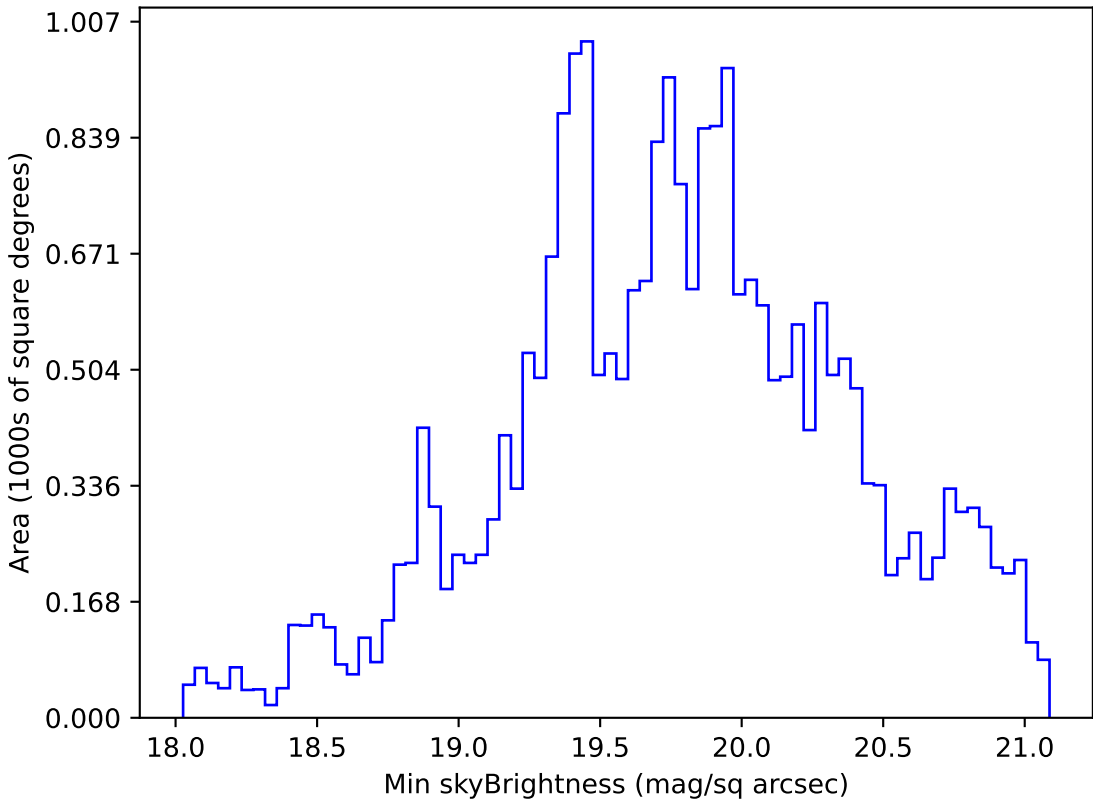
too_elab_heavy_r32_d3_gz_v3.4_10yrs Yr 1 r band: Min skyBrightness
