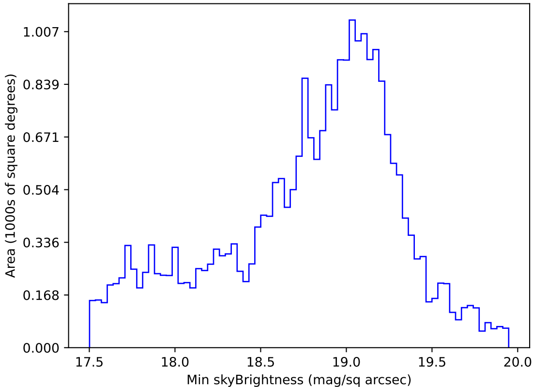
too_elab_heavy_r32_d3_gz_v3.4_10yrs Yr 1 i band: Min skyBrightness
