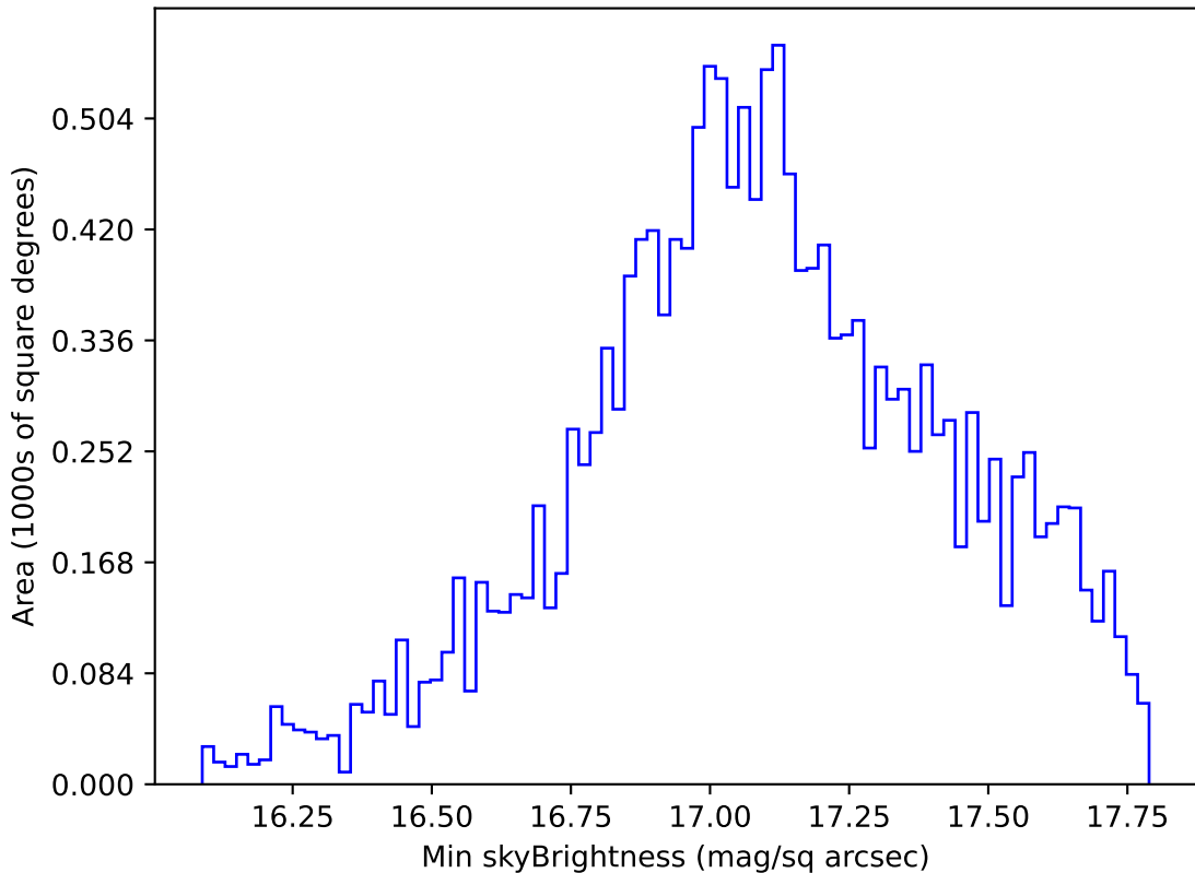
too_elab_heavy_r32_d3_gz_v3.4_10yrs WFD y band: Min skyBrightness
