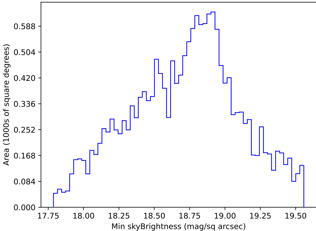
too_elab_heavy_r32_d3_gz_v3.4_10yrs WFD r band: Min skyBrightness
