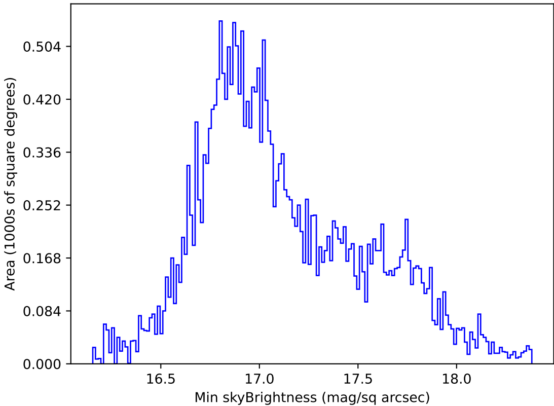
too_elab_heavy_r32_d3_gz_v3.4_10yrs All sky all bands: Min skyBrightness
