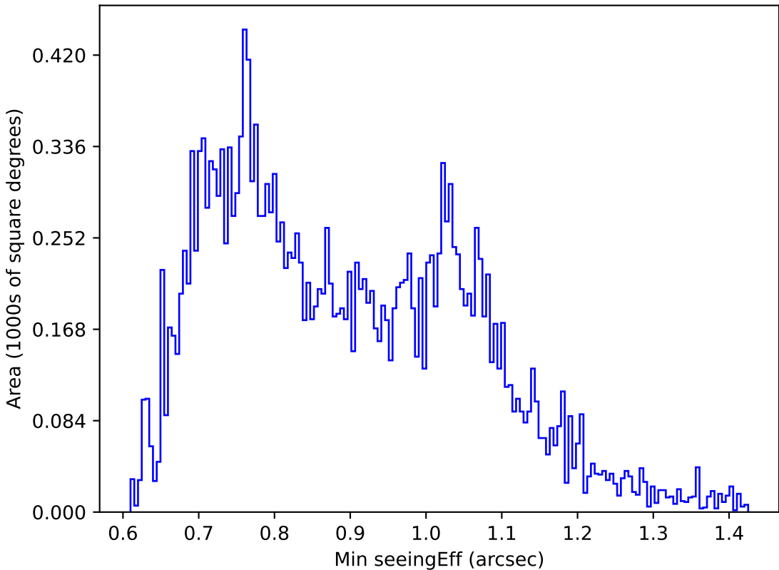
too_elab_heavy_r32_d3_gz_v3.4_10yrs Yr 1 u band: Min seeingEff
