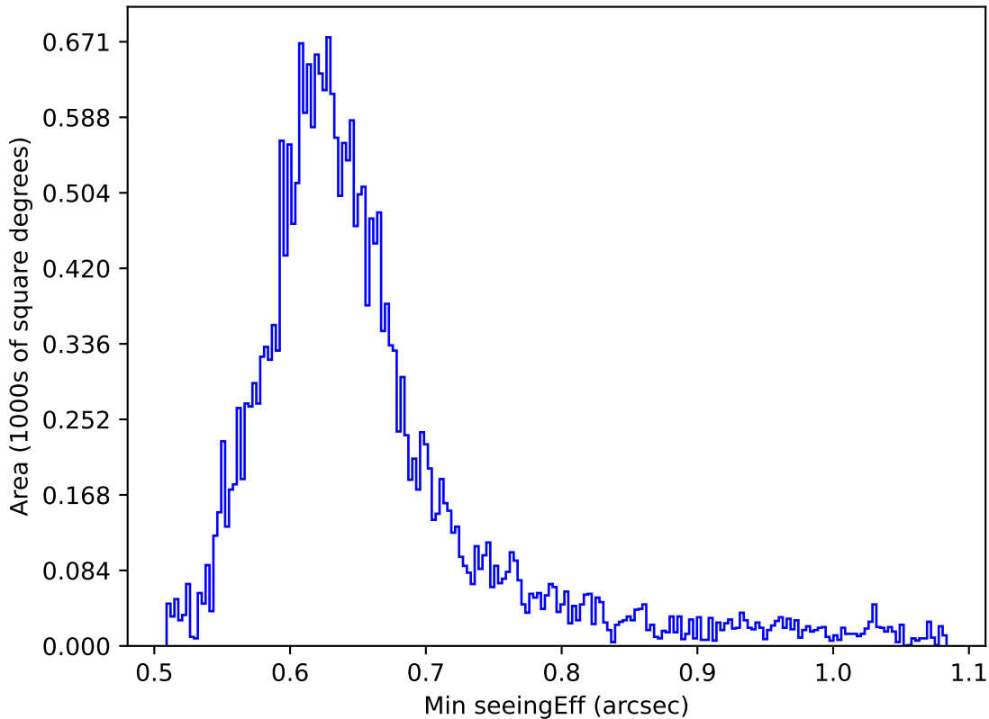
too_elab_heavy_r32_d3_gz_v3.4_10yrs Yr 1 all bands: Min seeingEff
