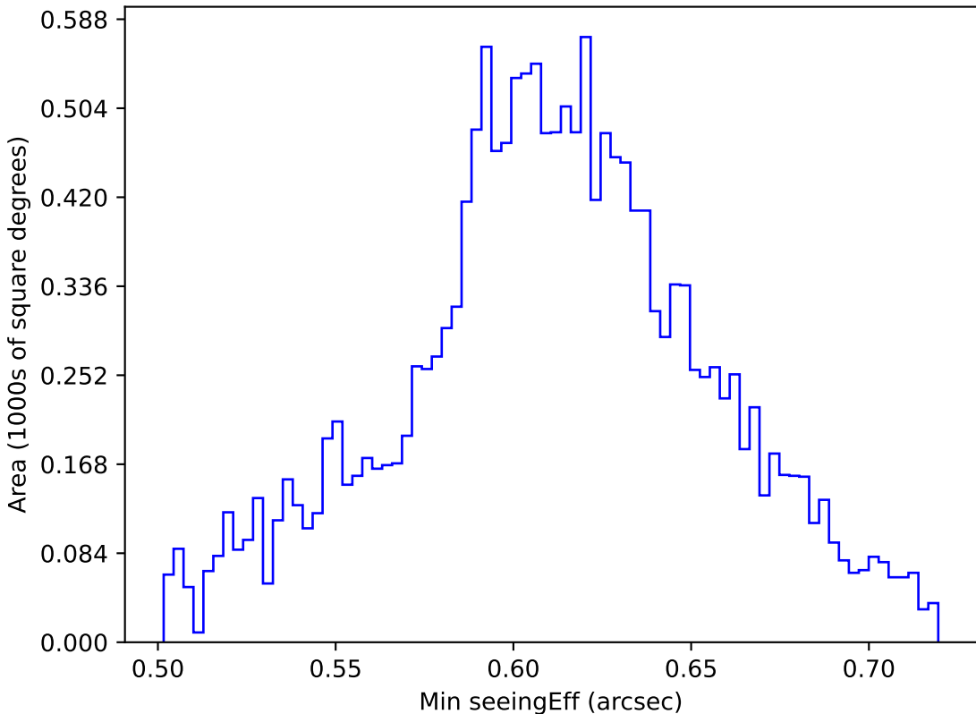
too_elab_heavy_r32_d3_gz_v3.4_10yrs WFD z band: Min seeingEff
