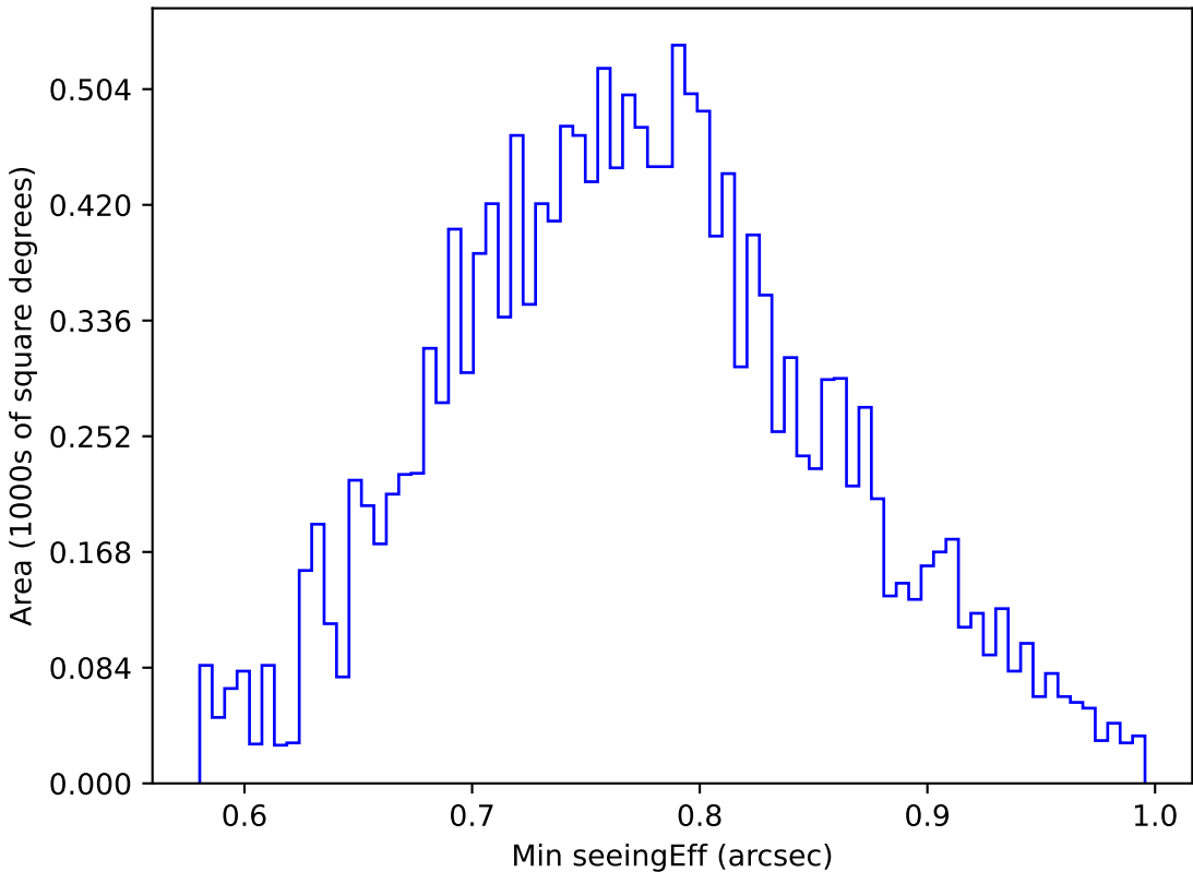
too_elab_heavy_r32_d3_gz_v3.4_10yrs WFD u band: Min seeingEff
