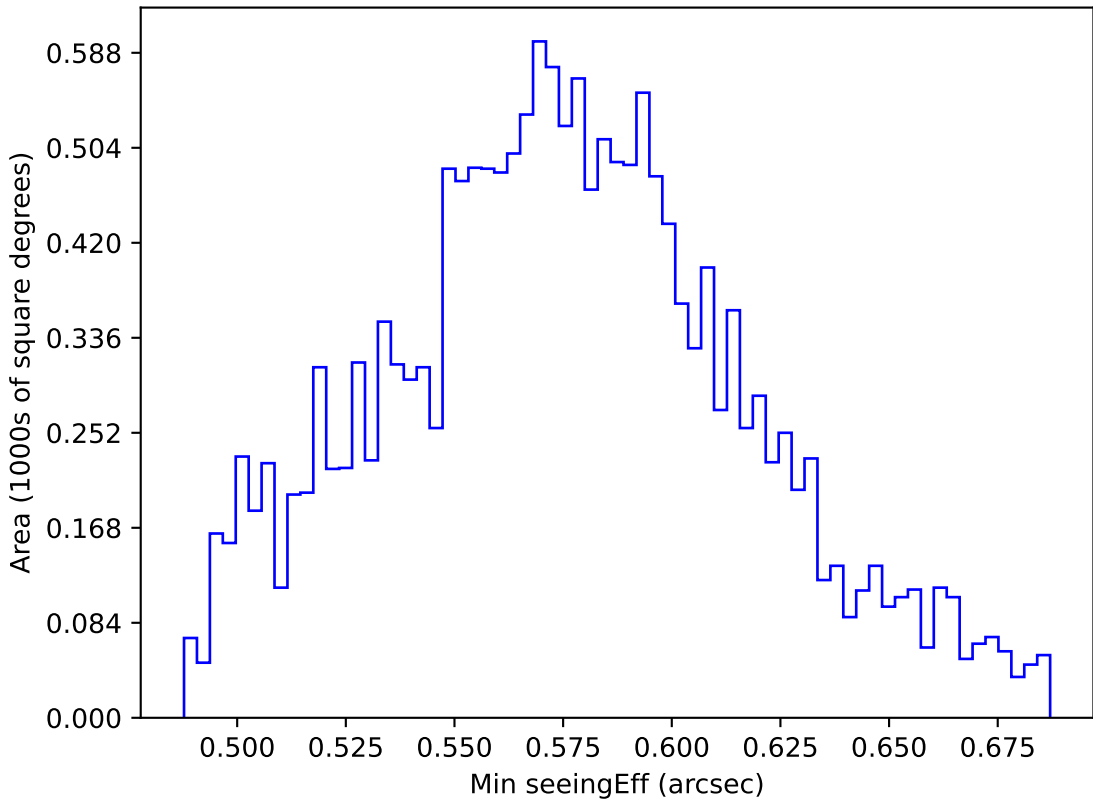
too_elab_heavy_r32_d3_gz_v3.4_10yrs WFD all bands: Min seeingEff
