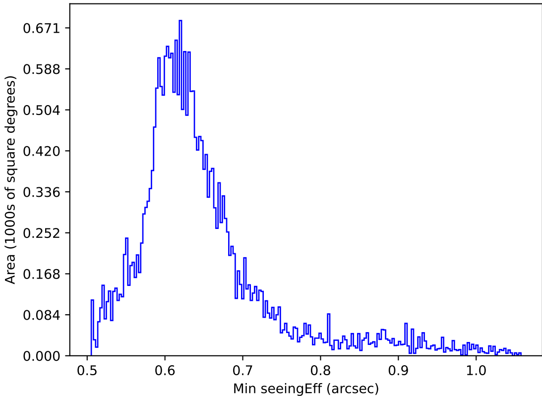
too_elab_heavy_r32_d3_gz_v3.4_10yrs All sky z band: Min seeingEff
