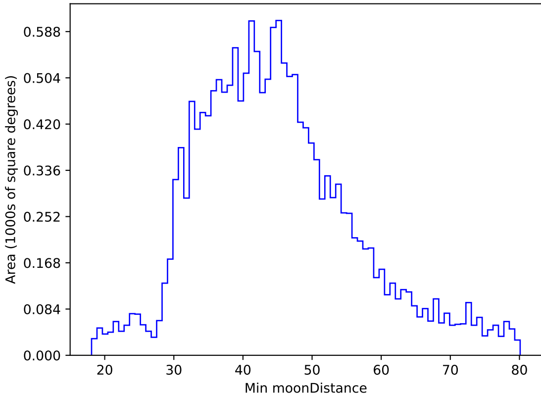
too_elab_heavy_r32_d3_gz_v3.4_10yrs WFD g band: Min moonDistance
