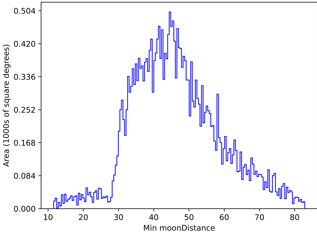
too_elab_heavy_r32_d3_gz_v3.4_10yrs All sky g band: Min moonDistance
