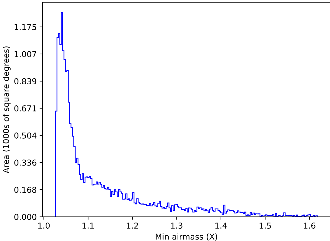
too_elab_heavy_r32_d3_gz_v3.4_10yrs Yr 1 y band: Min airmass
