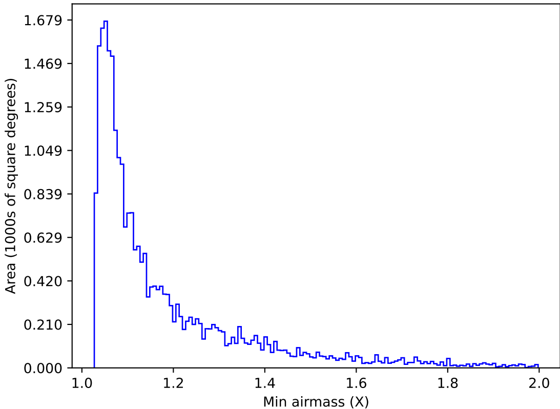
too_elab_heavy_r32_d3_gz_v3.4_10yrs Yr 1 g band: Min airmass
