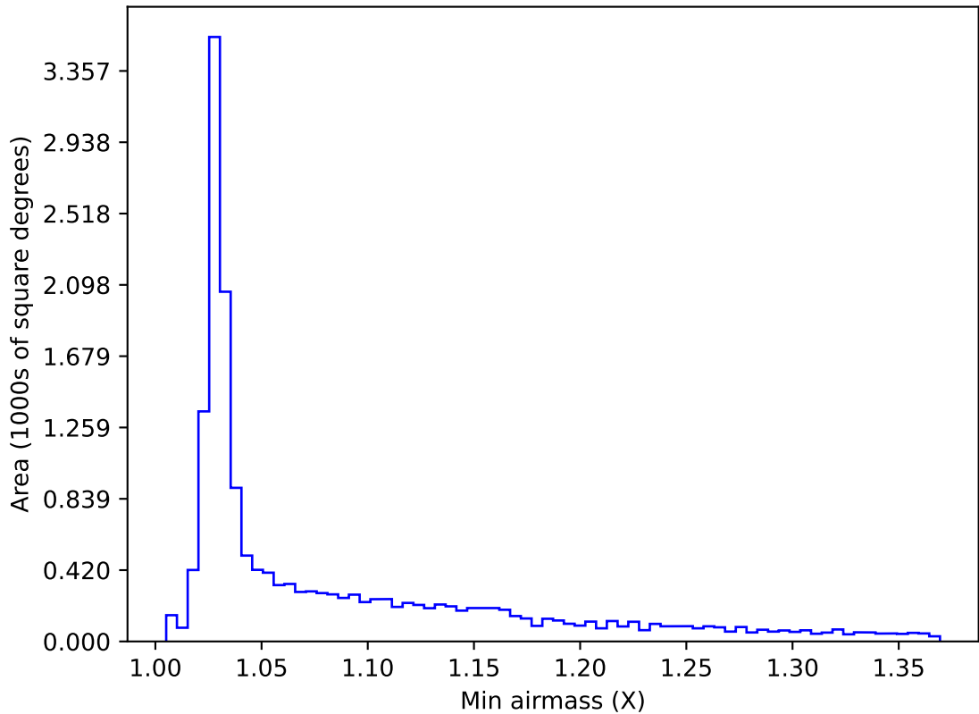
too_elab_heavy_r32_d3_gz_v3.4_10yrs WFD z band: Min airmass
