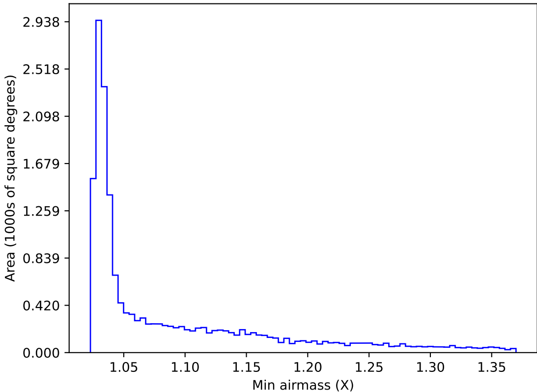
too_elab_heavy_r32_d3_gz_v3.4_10yrs WFD y band: Min airmass
