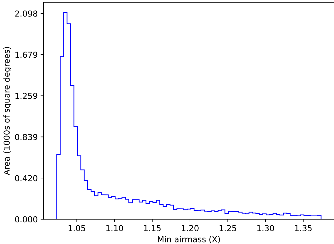
too_elab_heavy_r32_d3_gz_v3.4_10yrs WFD u band: Min airmass
