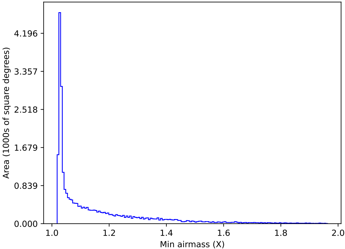
too_elab_heavy_r32_d3_gz_v3.4_10yrs All sky i band: Min airmass
