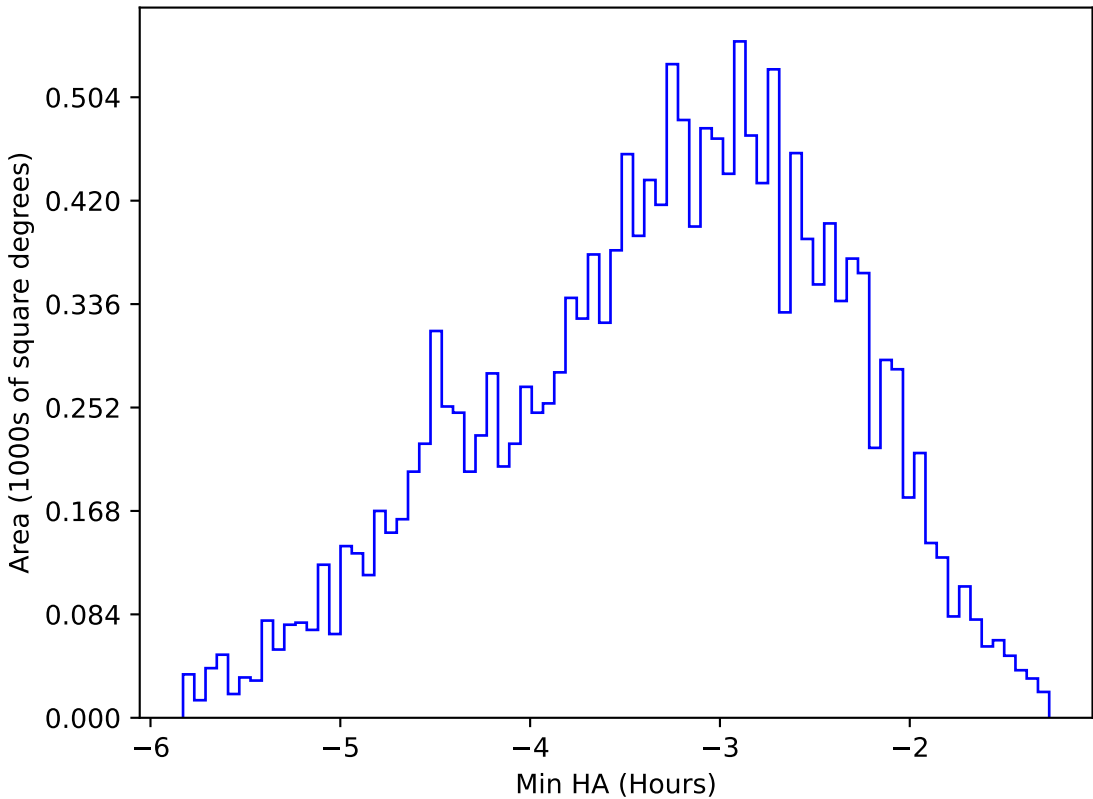
too_elab_heavy_r32_d3_gz_v3.4_10yrs WFD u band: Min HA
