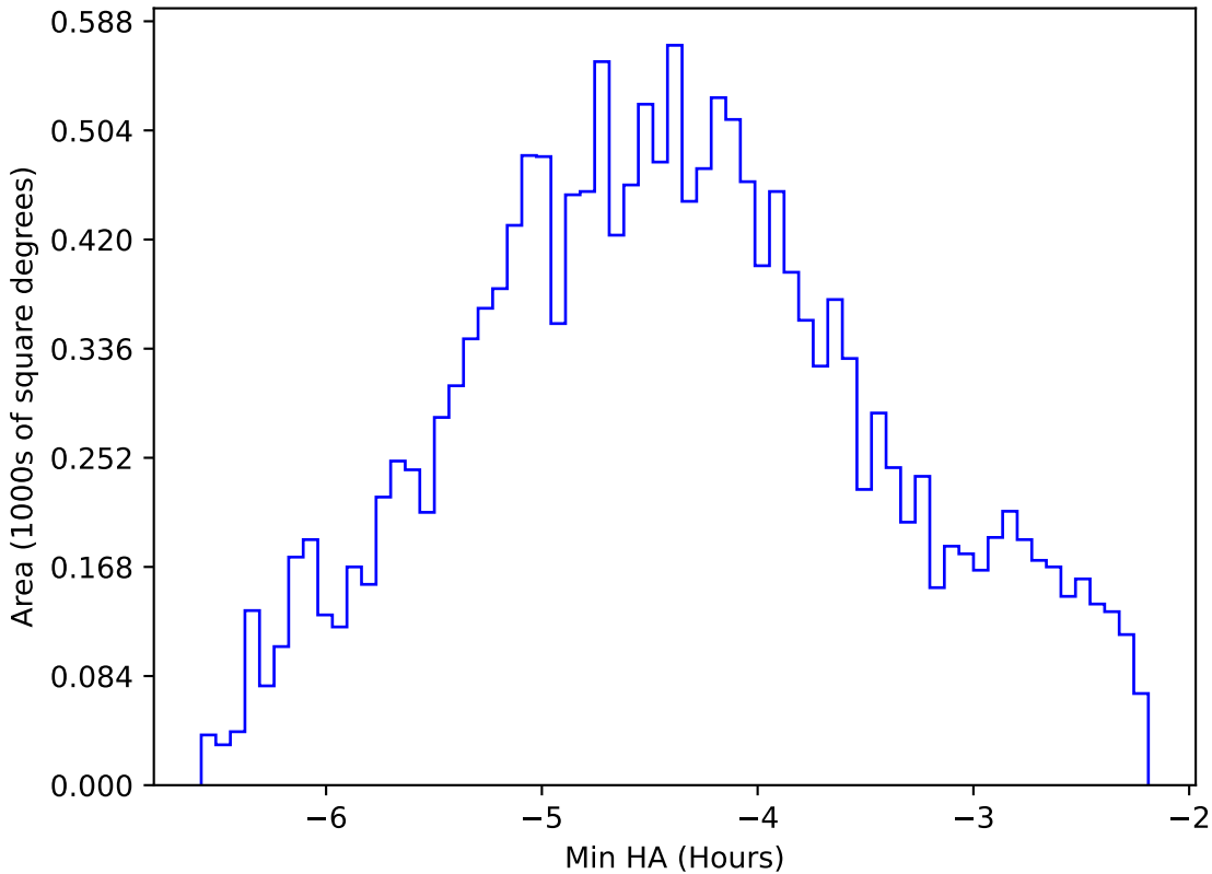
too_elab_heavy_r32_d3_gz_v3.4_10yrs WFD i band: Min HA
