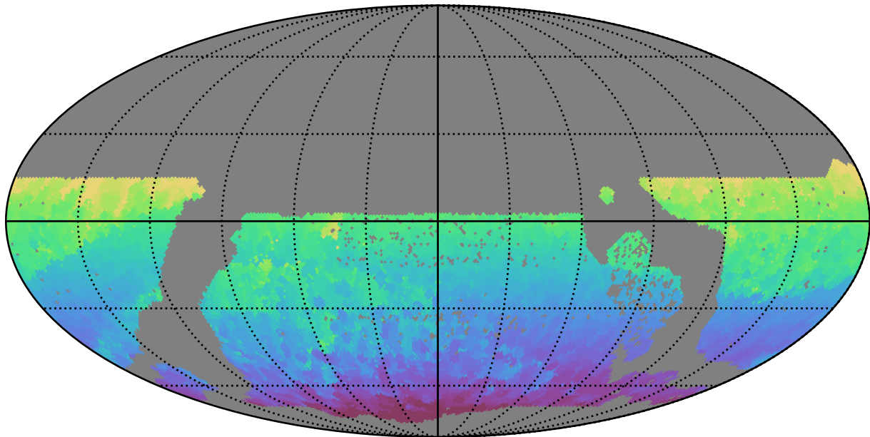
too_elab_heavy_r32_d3_gz_v3.4_10yrs WFD all bands: Min HA
