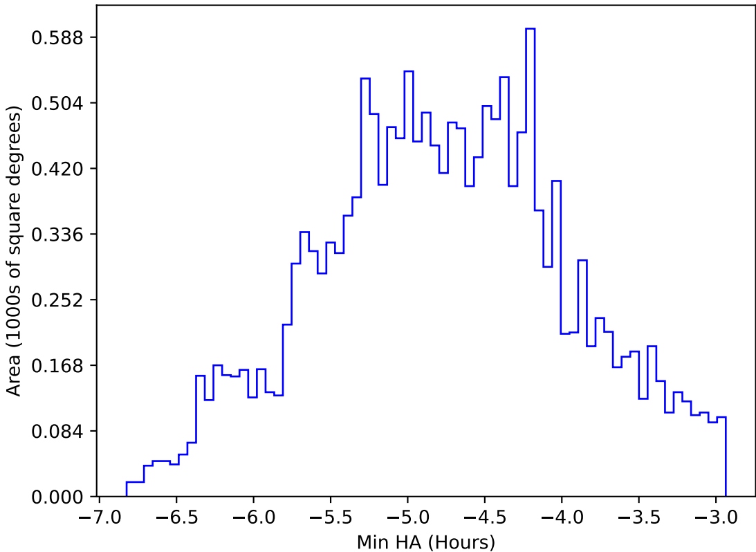
too_elab_heavy_r32_d3_gz_v3.4_10yrs WFD all bands: Min HA
