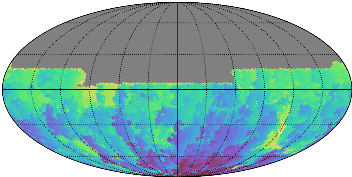
too_elab_heavy_r32_d3_gz_v3.4_10yrs All sky u band: Min HA
