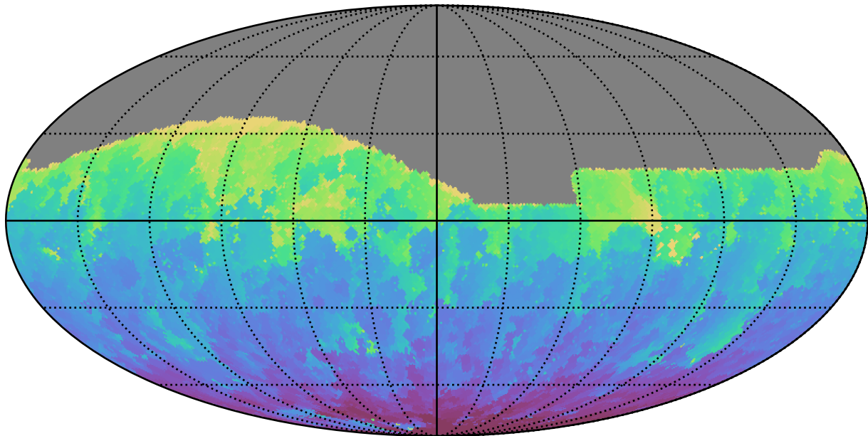
too_elab_heavy_r32_d3_gz_v3.4_10yrs All sky g band: Min HA
