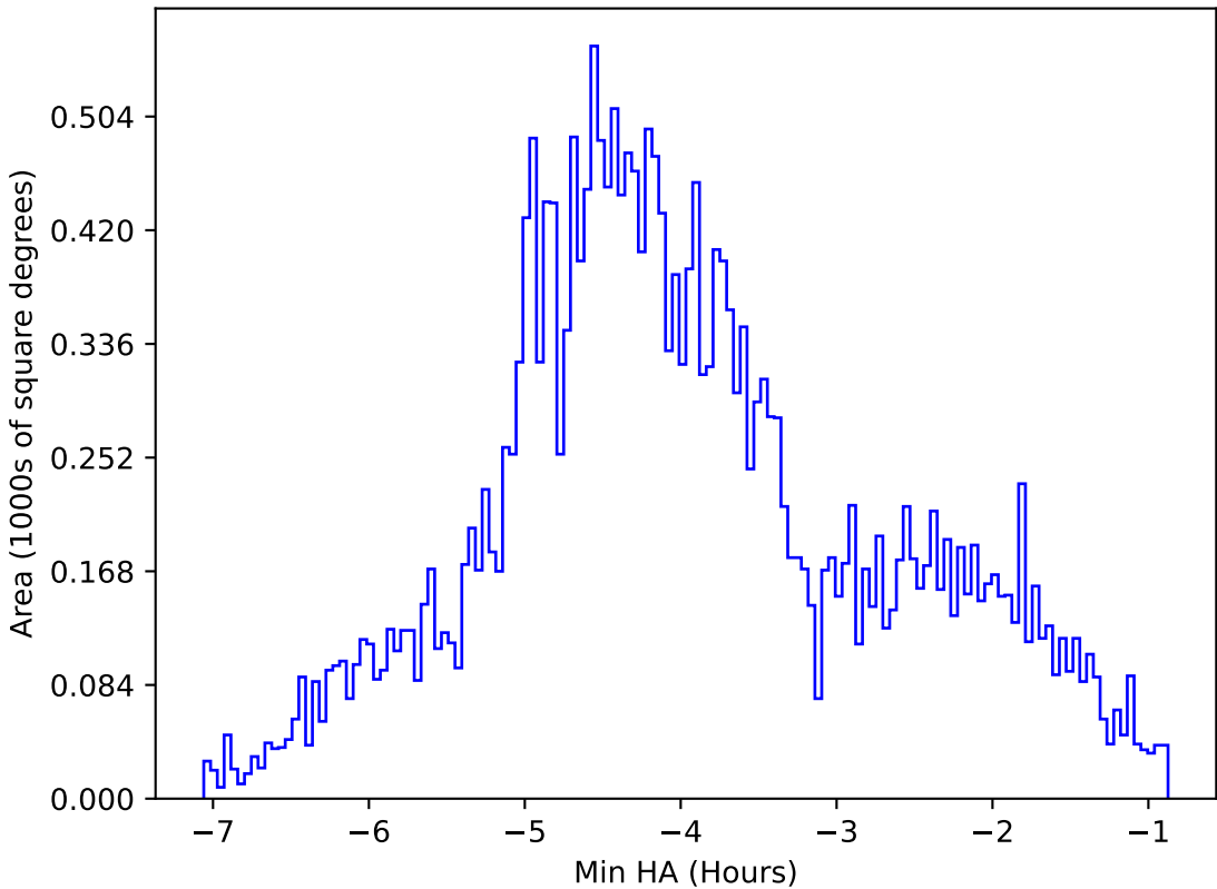
too_elab_heavy_r32_d3_gz_v3.4_10yrs All sky g band: Min HA
