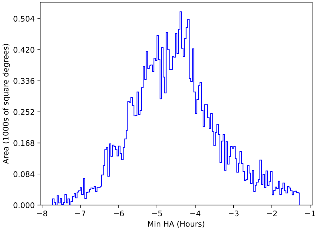
too_elab_heavy_r32_d3_gz_v3.4_10yrs All sky all bands: Min HA
