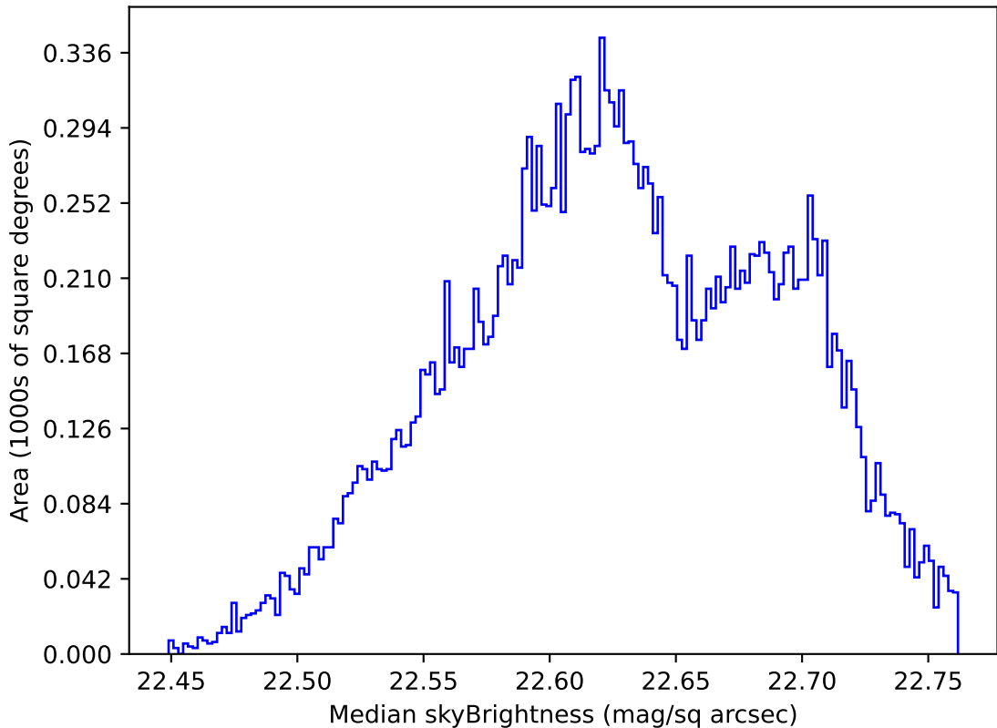
too_elab_heavy_r32_d3_gz_v3.4_10yrs Yr 1 u band: Median skyBrightness
