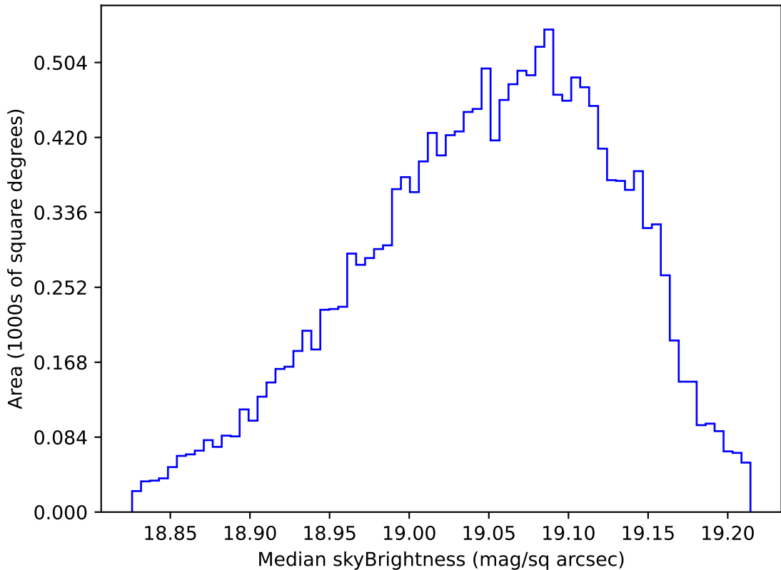
too_elab_heavy_r32_d3_gz_v3.4_10yrs WFD z band: Median skyBrightness
