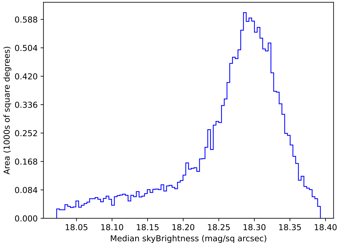
too_elab_heavy_r32_d3_gz_v3.4_10yrs WFD y band: Median skyBrightness
