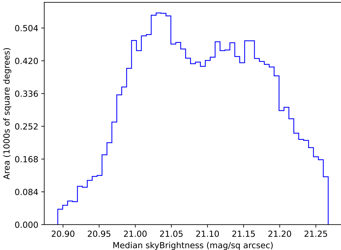
too_elab_heavy_r32_d3_gz_v3.4_10yrs WFD r band: Median skyBrightness
