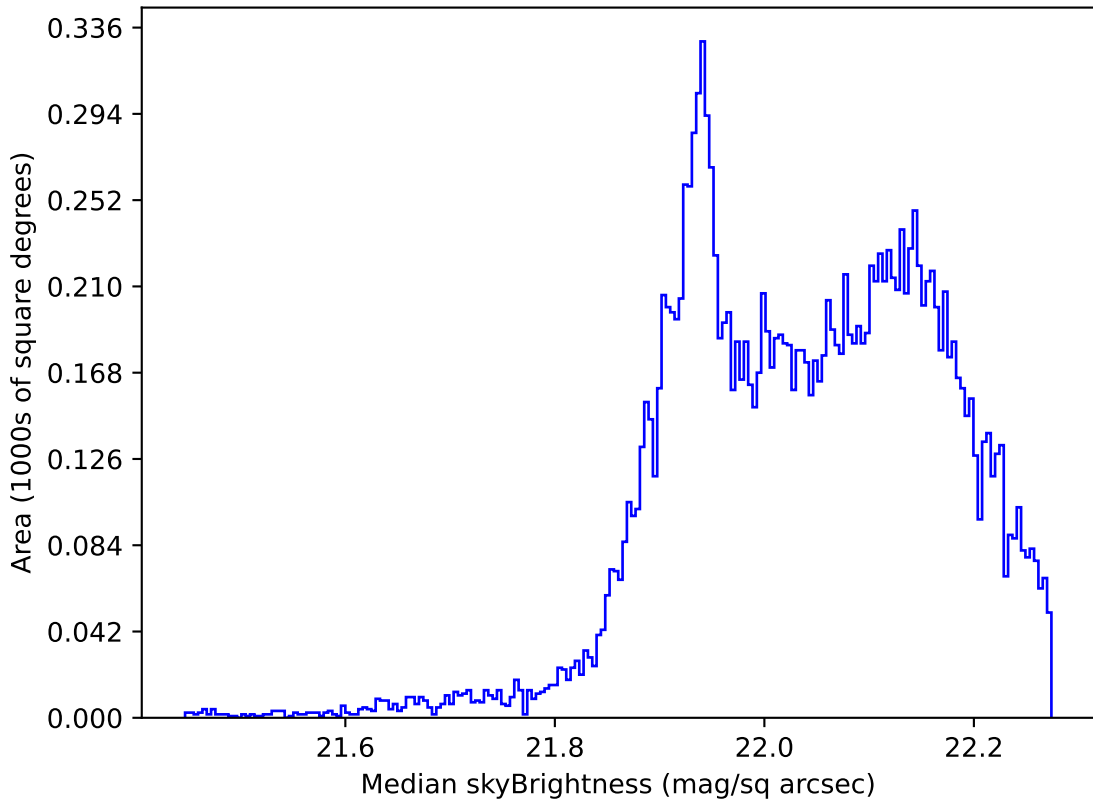
too_elab_heavy_r32_d3_gz_v3.4_10yrs WFD g band: Median skyBrightness
