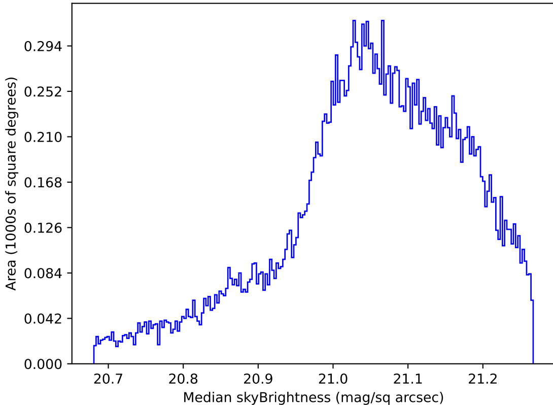
too_elab_heavy_r32_d3_gz_v3.4_10yrs All sky r band: Median skyBrightness
