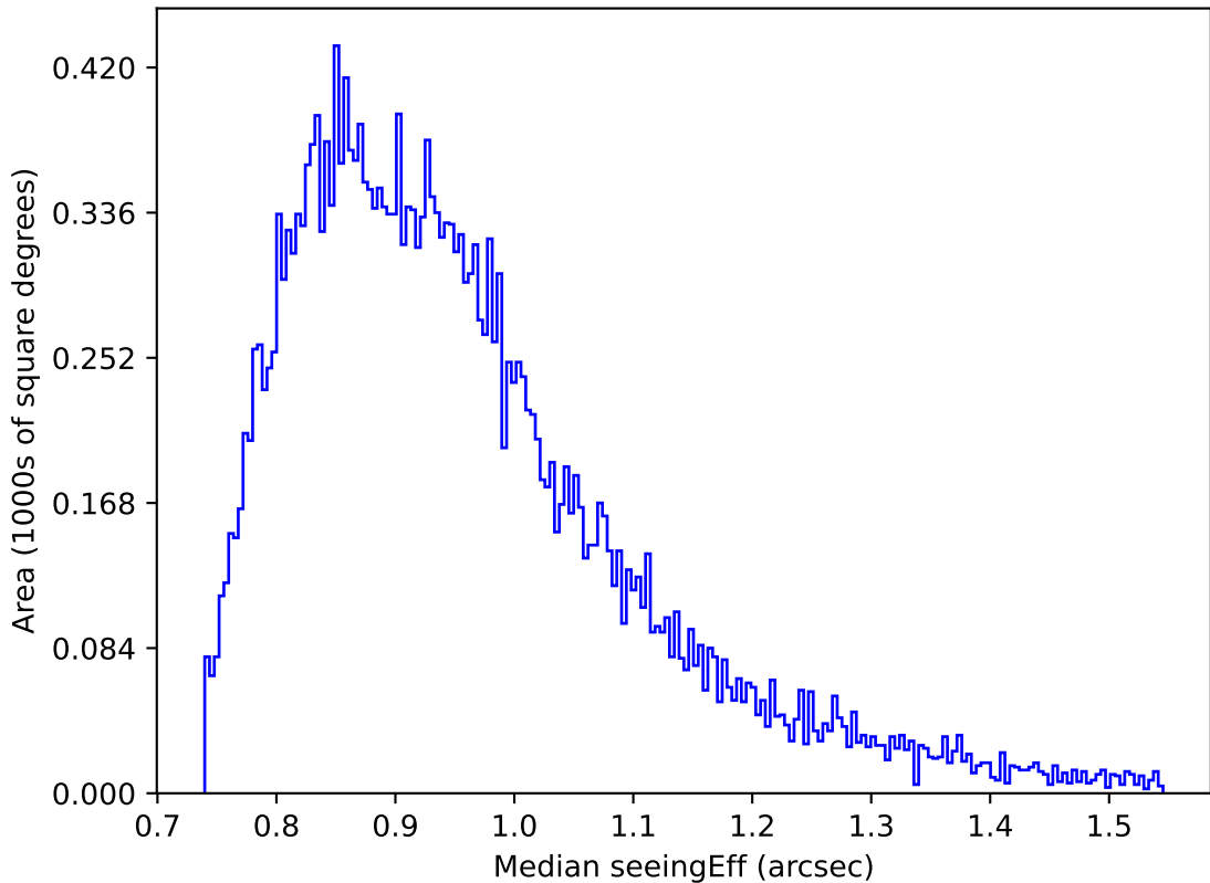
too_elab_heavy_r32_d3_gz_v3.4_10yrs Yr 1 i band: Median seeingEff
