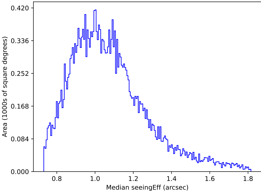
too_elab_heavy_r32_d3_gz_v3.4_10yrs Yr 1 g band: Median seeingEff
