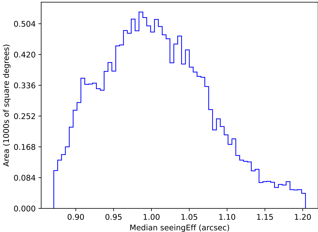
too_elab_heavy_r32_d3_gz_v3.4_10yrs WFD z band: Median seeingEff
