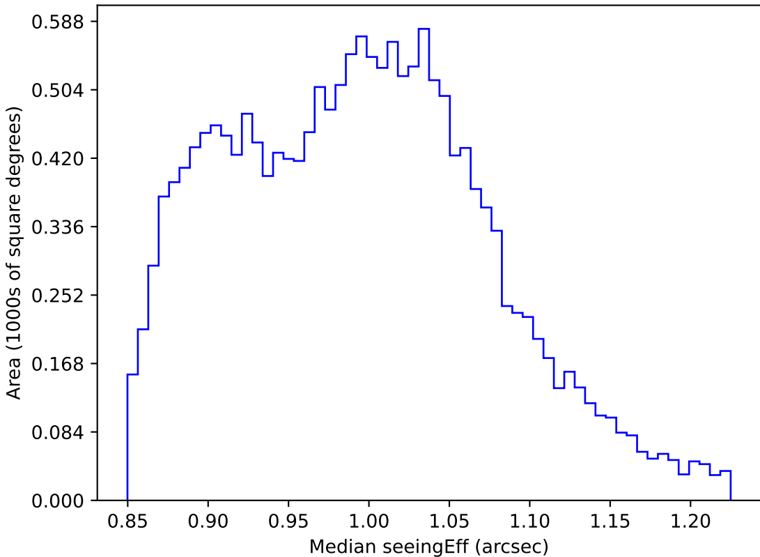
too_elab_heavy_r32_d3_gz_v3.4_10yrs WFD i band: Median seeingEff
