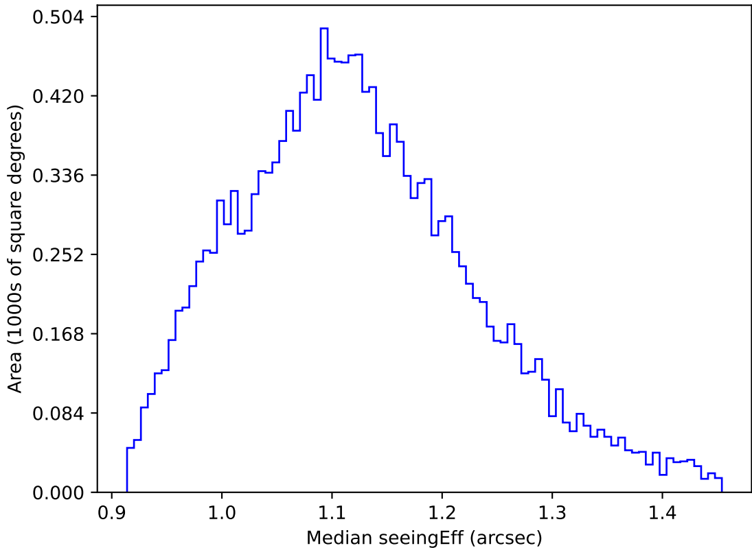
too_elab_heavy_r32_d3_gz_v3.4_10yrs WFD g band: Median seeingEff
