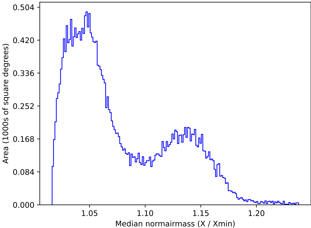
too_elab_heavy_r32_d3_gz_v3.4_10yrs All sky i band: Median normairmass
