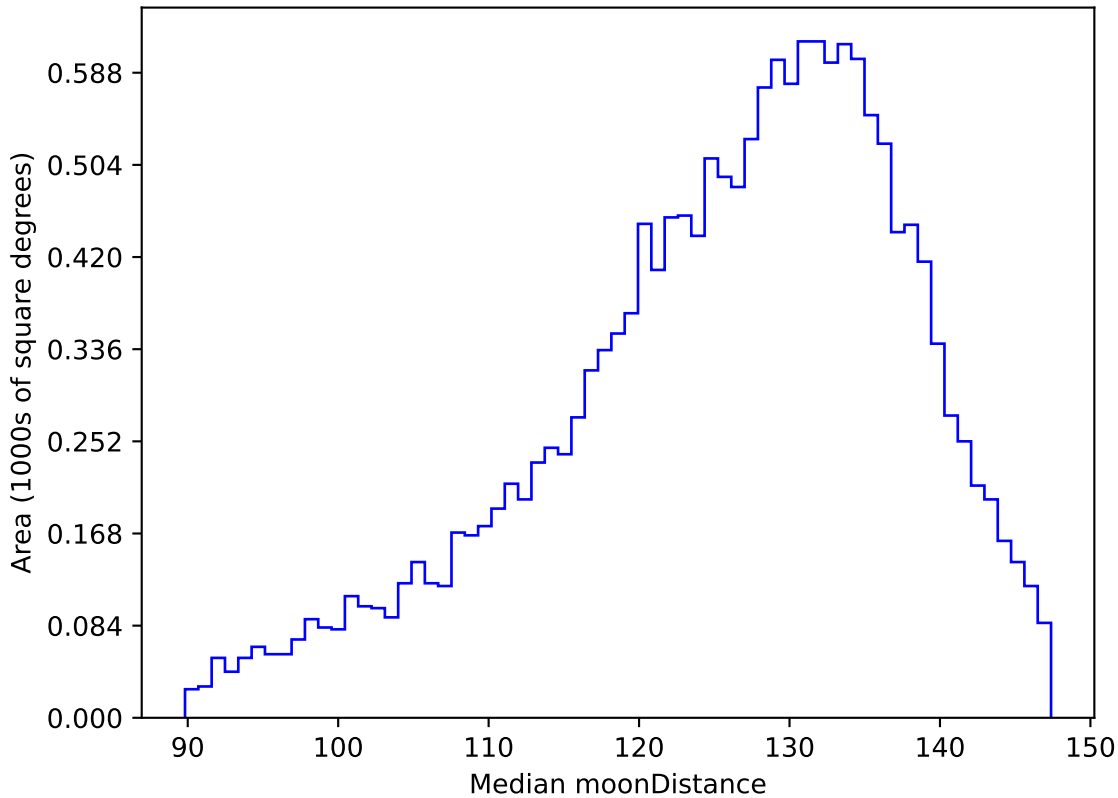
too_elab_heavy_r32_d3_gz_v3.4_10yrs WFD u band: Median moonDistance
