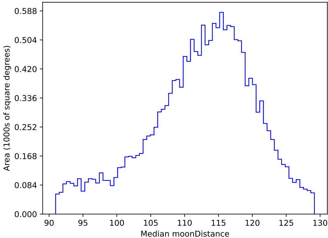
too_elab_heavy_r32_d3_gz_v3.4_10yrs WFD r band: Median moonDistance
