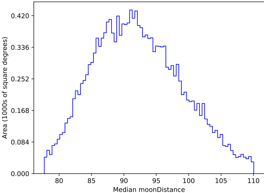
too_elab_heavy_r32_d3_gz_v3.4_10yrs WFD i band: Median moonDistance
