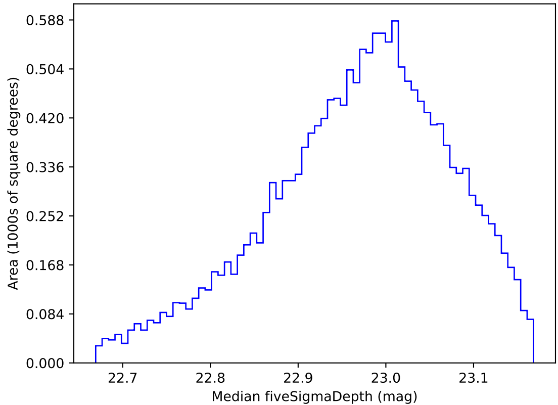
too_elab_heavy_r32_d3_gz_v3.4_10yrs WFD z band: Median fiveSigmaDepth
