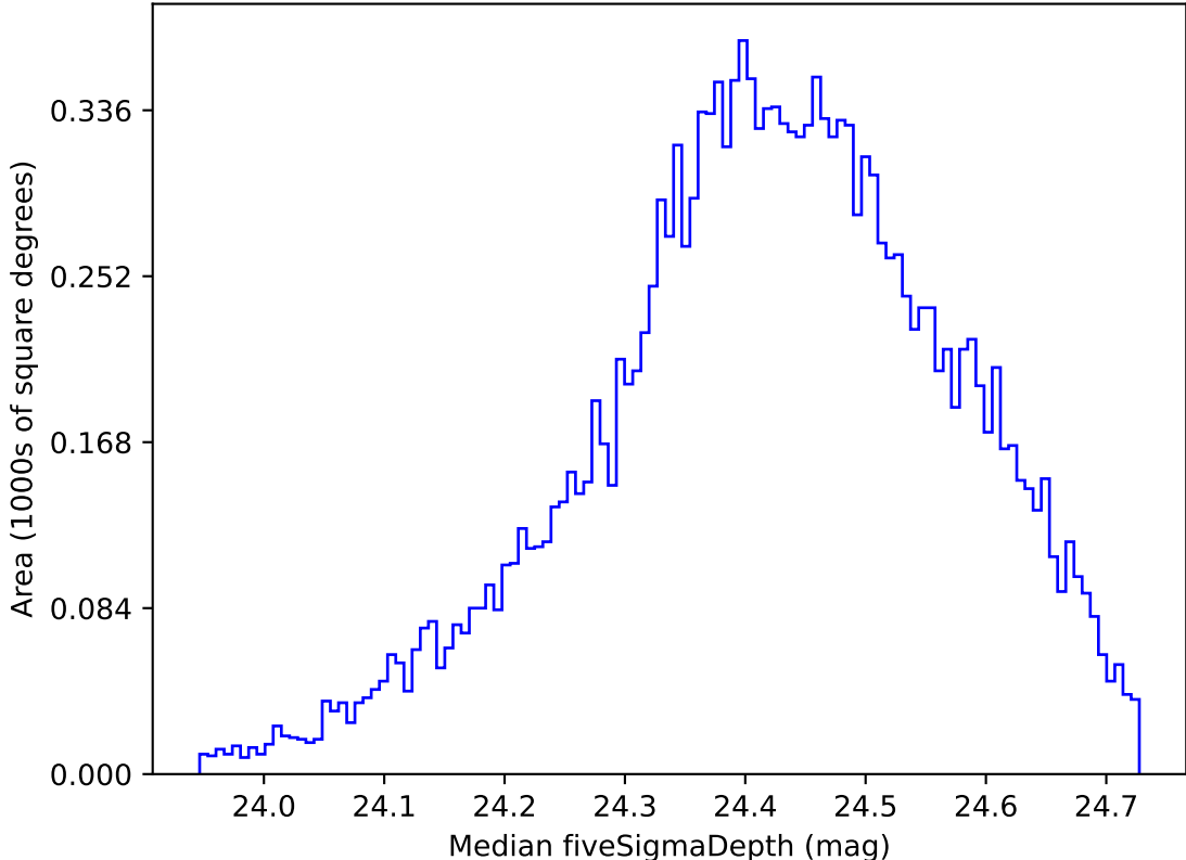
too_elab_heavy_r32_d3_gz_v3.4_10yrs WFD g band: Median fiveSigmaDepth
