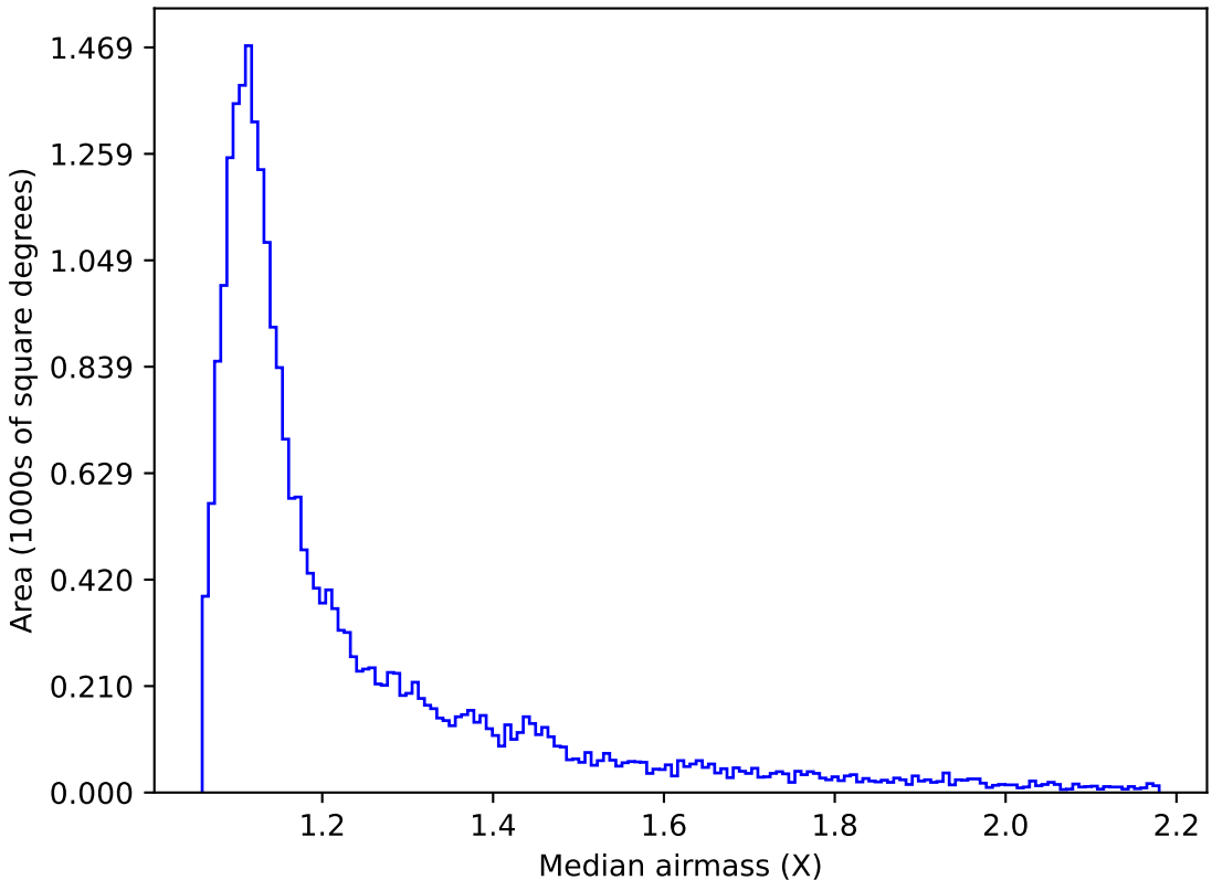
too_elab_heavy_r32_d3_gz_v3.4_10yrs Yr 1 i band: Median airmass
