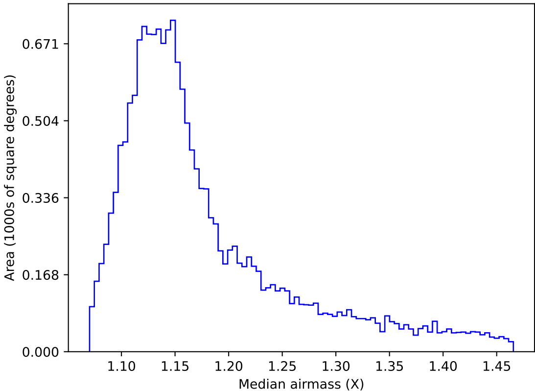
too_elab_heavy_r32_d3_gz_v3.4_10yrs WFD u band: Median airmass
