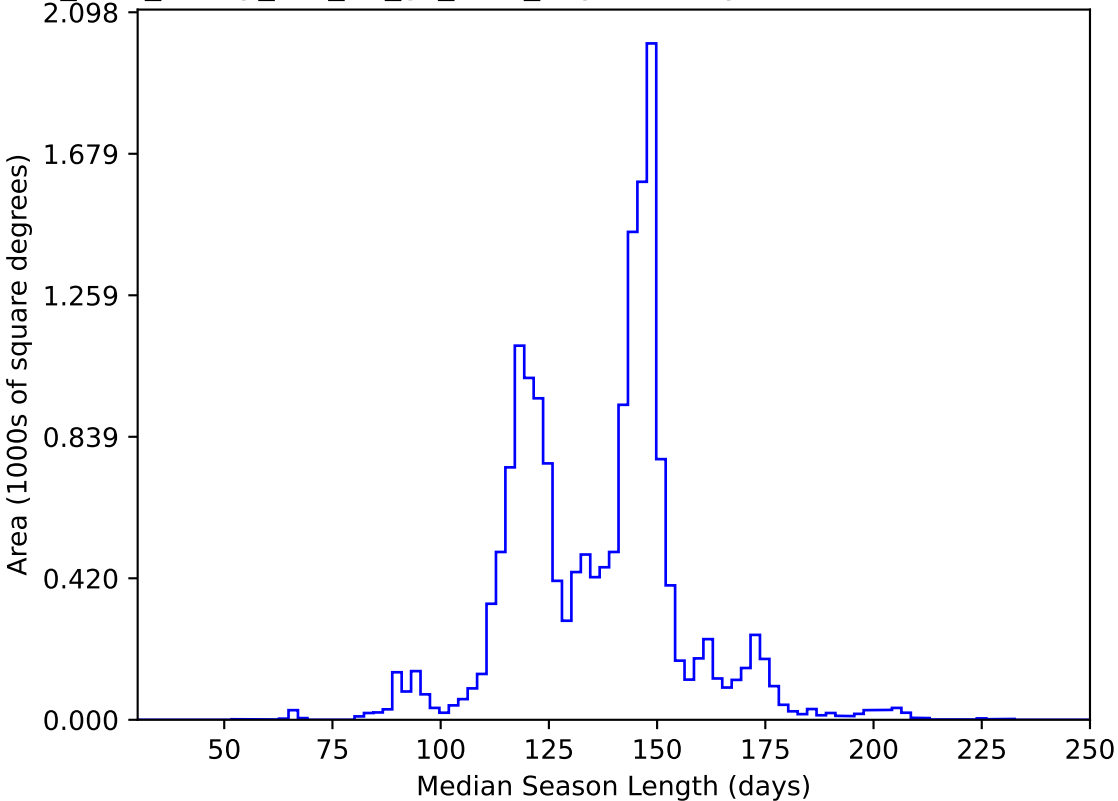
too_elab_heavy_r32_d3_gz_v3.4_10yrs WFD y band: Median Season Length
